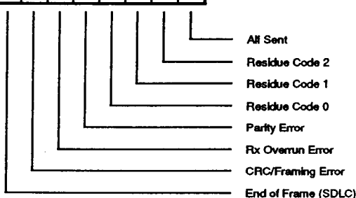
Read Register 1
