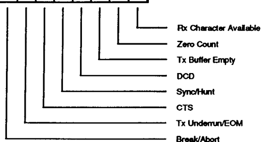
Read Register 0
