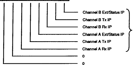
Read Register 3
