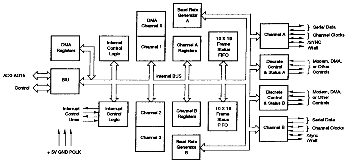
Figure 3. Block Diagram of ISCC Architecture
