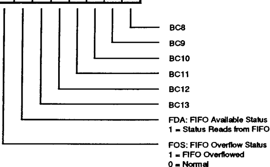
Read Register 7 *
