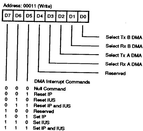
Figure 15. Interrupt Command/Register
