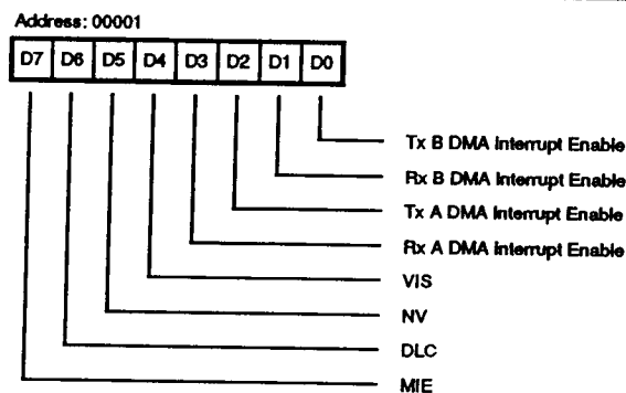
Figure 13. Interrupt Control Register
