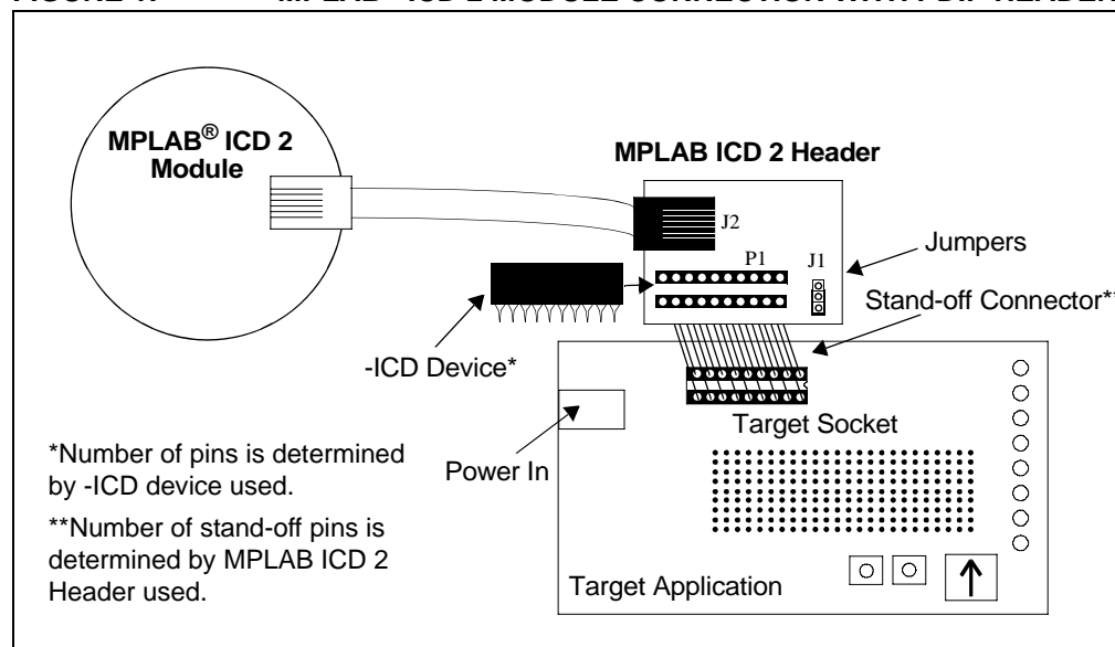
FIGURE 1: MPLAB® ICD 2 MODULE CONNECTION WITH PDIP HEADER
