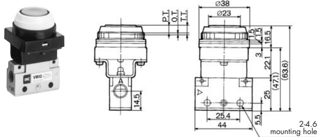
Replacement operator head VM-33A
