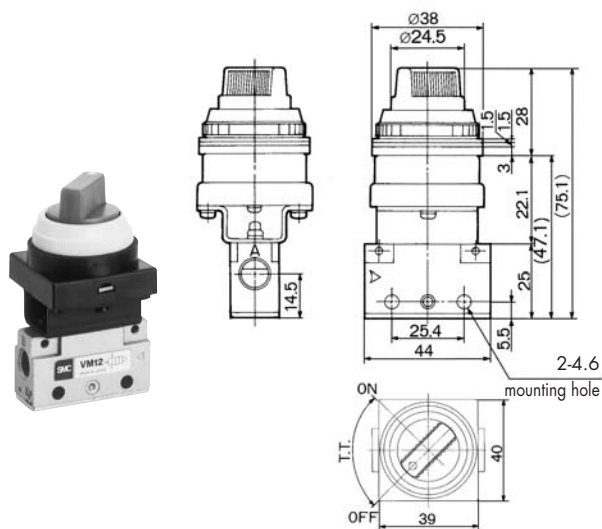
Replacement operator head VM-34A*
