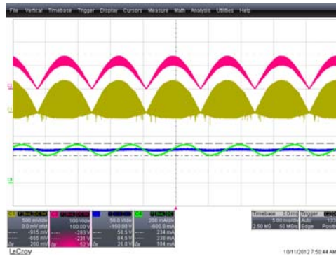
Figure 11. V_{IN} = 90 V_{AC} / 60 \text{ Hz} , Operation Waveforms at LED (70 V / 300 mA); C1 [V CS ], C2 [V IN ], C3 [V OUT ], C4 [I OUT ]
