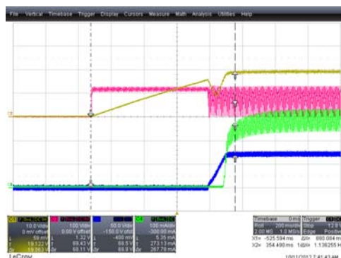
Figure 7. V_{IN} = 90\text{ V}_{AC} / 60\text{ Hz} , Startup Time at LED (70 V / 300 mA); C1 [ V_{DD} ], C2 [ V_{IN} ], C3 [ V_{OUT} ], C4 [ I_{OUT} ]
