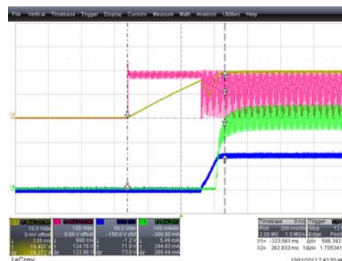
Figure 8. V_{IN} = 120\text{ V}_{AC} / 60\text{ Hz} Startup Time at LED (70 V / 300 mA); C1 [ V_{DD} ], C2 [ V_{IN} ], C3 [ V_{OUT} ], C4 [ I_{OUT} ]
