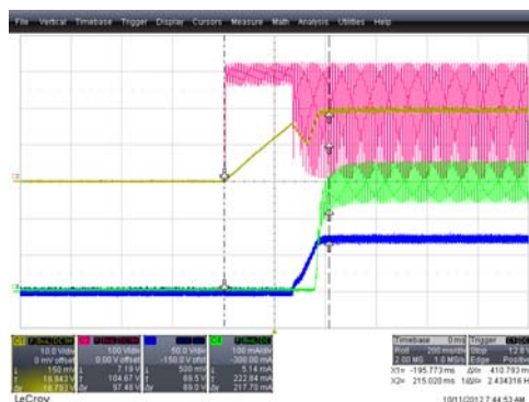
Figure 9. V_{IN} = 230\text{ V}_{AC} / 50\text{ Hz} , Startup Time at LED (70 V / 300 mA); C1 [ V_{DD} ], C2 [ V_{IN} ], C3 [ V_{OUT} ], C4 [ I_{OUT} ]
