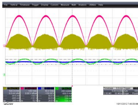
Figure 13. V_{IN} = 230 V_{AC} / 50 \text{ Hz} , Operation Waveforms at LED (70 V / 300 mA); C1 [V CS ], C2 [V IN ], C3 [V OUT ], C4 [I OUT ]
