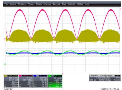
Figure 14. V_{IN} = 265 V_{AC} / 50 \text{ Hz} , Operation Waveforms at LED (70 V / 300 mA); C1 [V CS ], C2 [V IN ], C3 [V OUT ], C4 [I OUT ]
