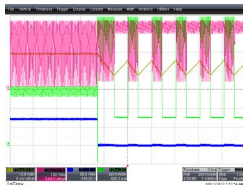
Figure 17. V_{IN} = 265 V_{AC} / 50 \text{ Hz} , Short-LED; C1 [ V_{DD} ], C2 [ V_{IN} ], C3 [ V_{OUT} ], C4 [ I_{OUT} ]
