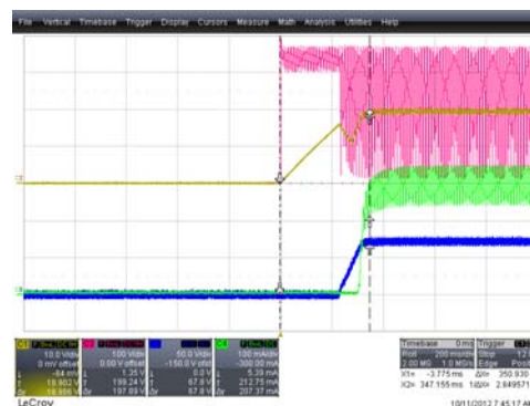
Figure 10. V_{IN} = 265\text{ V}_{AC} / 50\text{ Hz} , Startup Time at LED (70 V / 300 mA); C1 [ V_{DD} ], C2 [ V_{IN} ], C3 [ V_{OUT} ], C4 [ I_{OUT} ]
