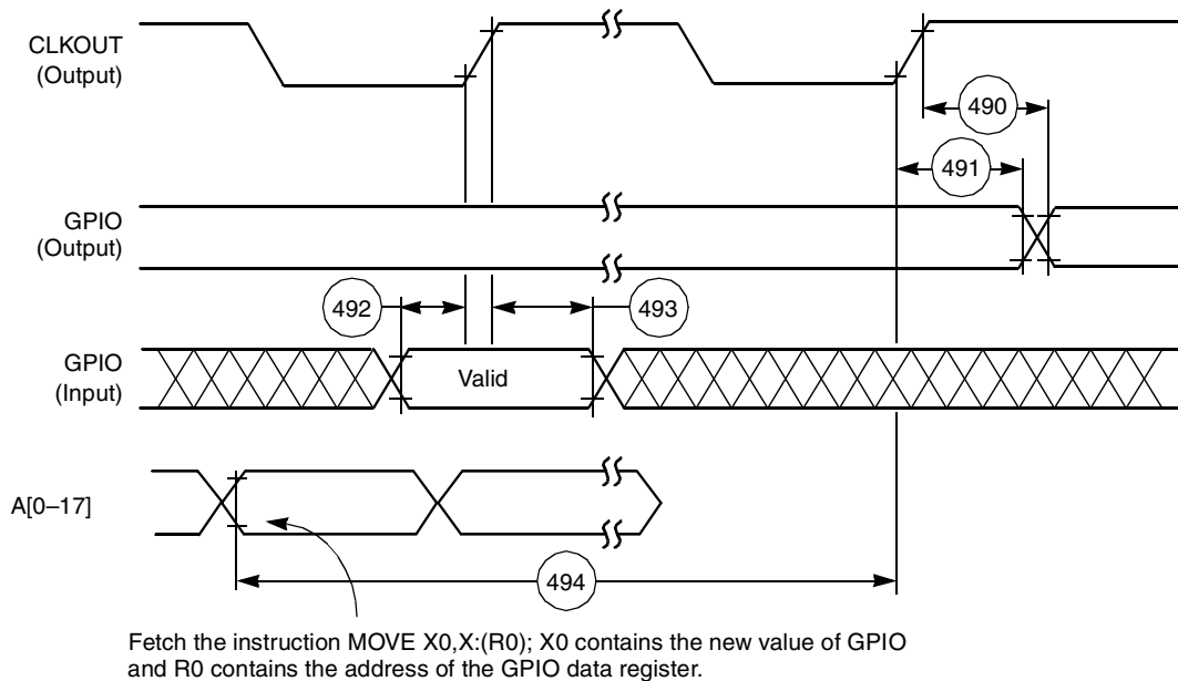
Figure 2-34. GPIO Timing
