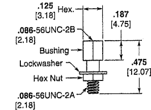
Jackpost Assembly (P) 096-0002-0009 M83513/5-07 P mates with K,KM, L,LM, Q,QM and R,RM Jackscrew Assemblies.
