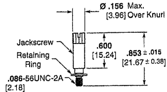
Jackscrew Assembly High Profile (K) 096-0002-0010 M83513/5-06 (KM) 096-0002-0084
