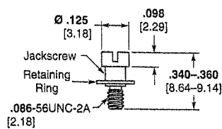
Jackscrew Assembly Low Profile (L) 096-0002-0011 M83513/5-05 (LM) 096-0002-0085
