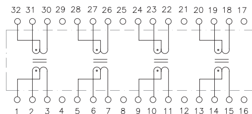
Schematic A
