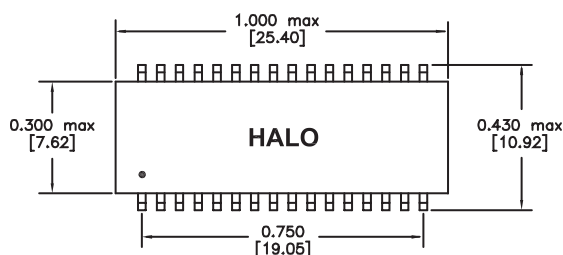
NU Package
