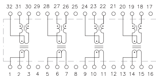
Schematic B
