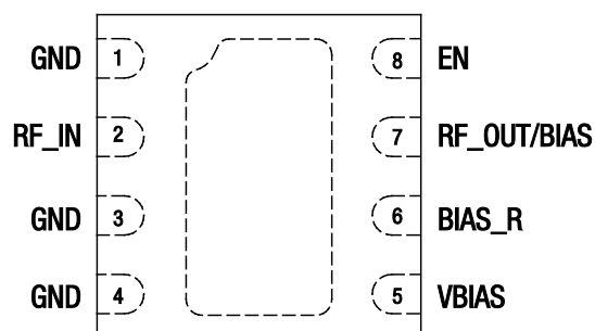
Figure 2. SKY65047-360LF Pinout – 8-Pin DFN (Top View)
