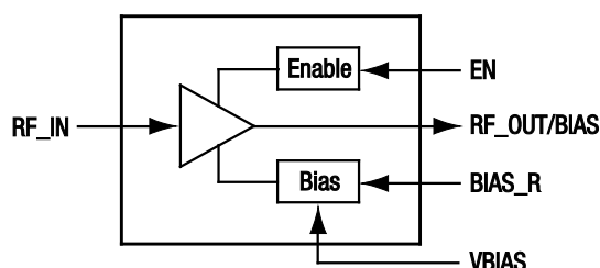
Figure 1. SKY65047-360LF Block Diagram
