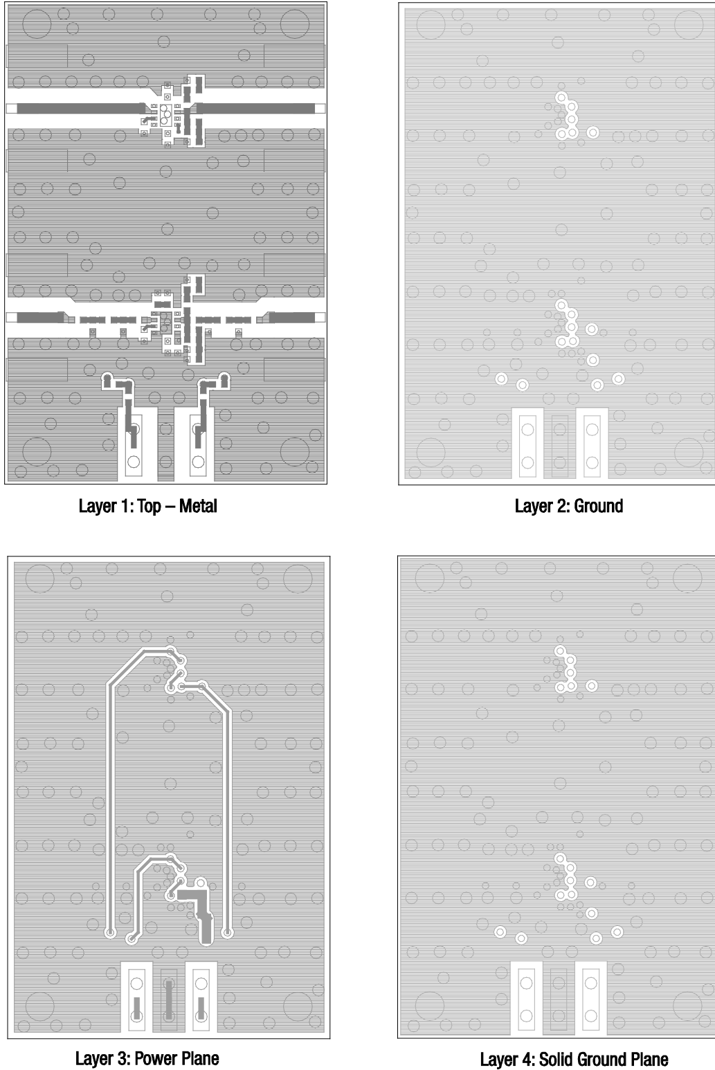
Figure 15. SKY65047-360LF Evaluation Board Layer Detail (915 MHz)
