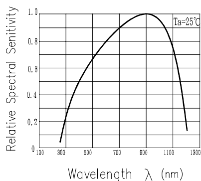
Fig.5 Spectral Sensitivity
