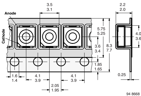
Figure 10. Tape dimensions in mm for PLCC-2
