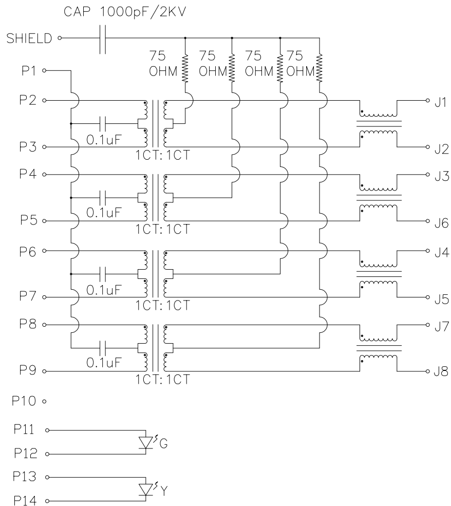
SCHEMATIC
