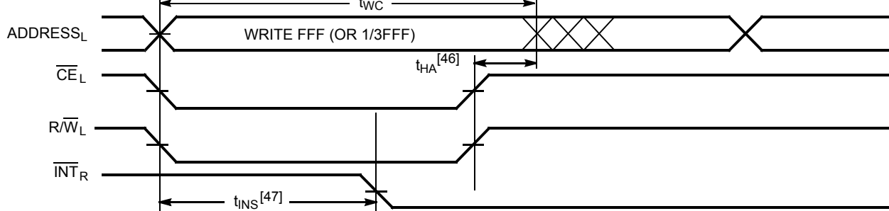
Figure 15. Interrupt Timing Diagram
