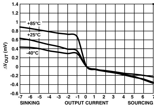
FIGURE 63. LOAD REGULATION
