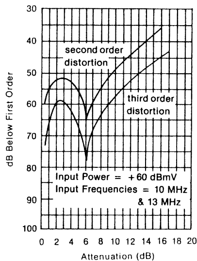
DISTORTION ATTENUATION
