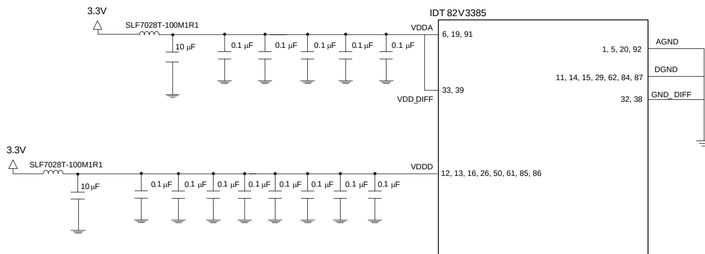
Figure 14. IDT82V3385 Power Decoupling Scheme
