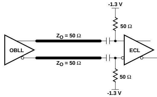
C) DIFFERENTIAL DRIVE O-BLL TO ECL
