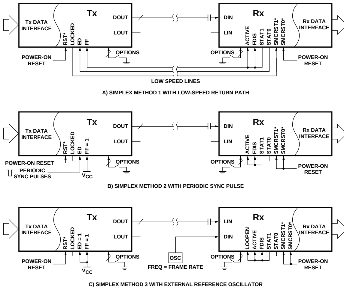
Figure 17. Simplex Configurations.
