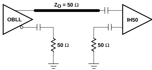
A) SINGLE-ENDED DRIVE O-BLL TO I-H50
