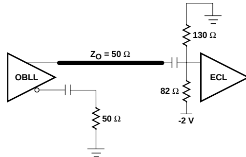
D) SINGLE-ENDED DRIVE O-BLL TO ECL
