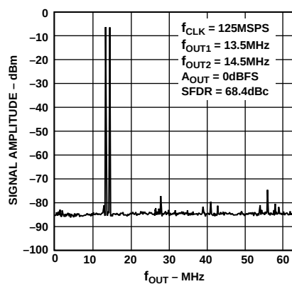
Figure 15. Dual-Tone SFDR
