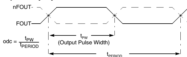
Figure 7: Output Duty Cycle
