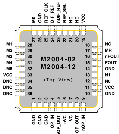
Figure 1: Pin Assignment
