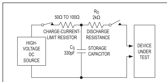
Figure 16. ISO 10605 Contact Discharge ESD Test Circuit
