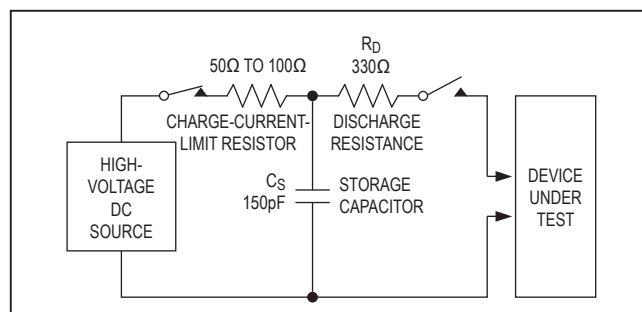
Figure 14. IEC 61000-4-2 Contact Discharge ESD Test Circuit
