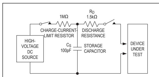
Figure 15. Human Body ESD Test Circuit
