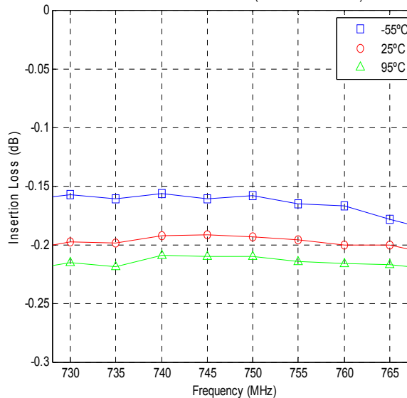
Insertion Loss for X3DC07E2S (Low Power Condition)
