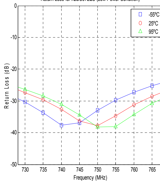
Return Loss for X3DC07E2S (Low Power Condition)
