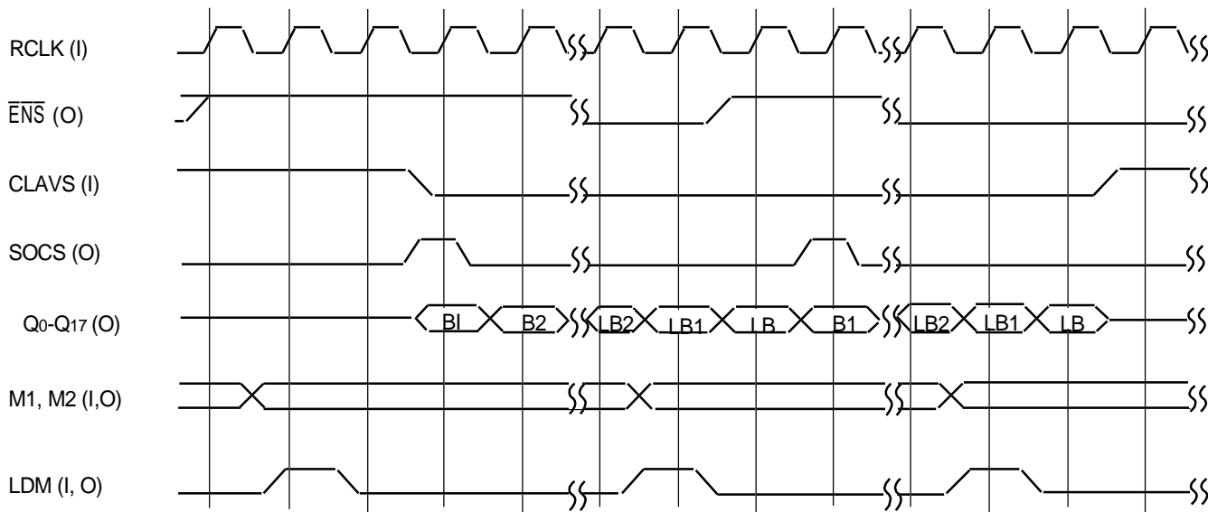
Figure 10e. Tx Mode—Output Timing
