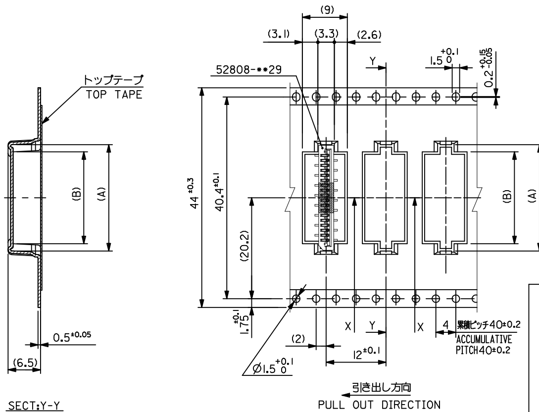
SECT:Y-Y
