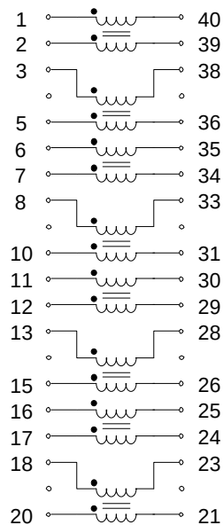
P/N F-1921V Schematic Diagram
