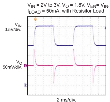
Line Transient
