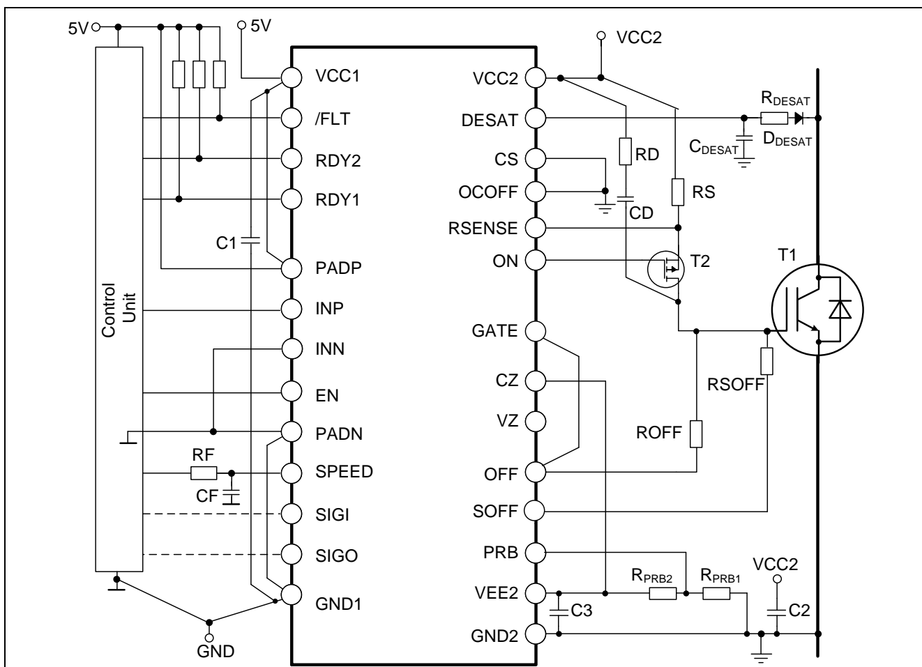
Figure 3 Typical application
