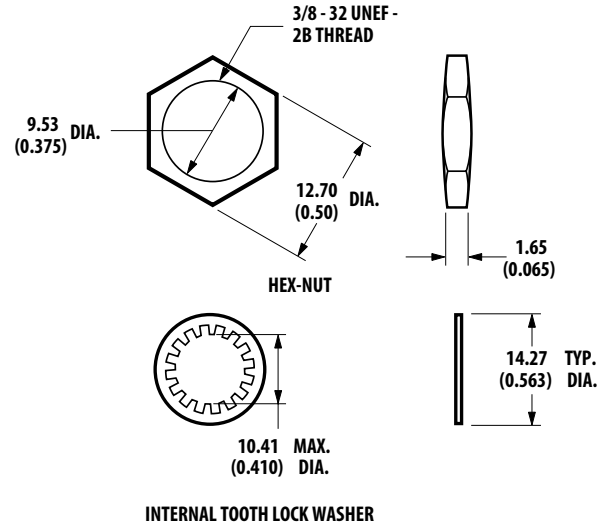
Figure 1. HFBR-4411Z mechanical dimensions
