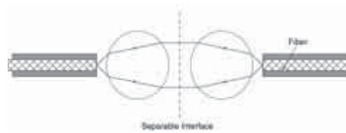
Expanded Beam Principle
