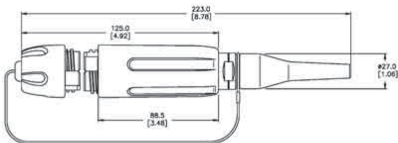
PRO BEAM Sr. Cable Connector, Plug
