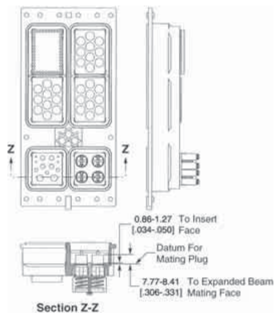
Typical Layout for Receptacle
