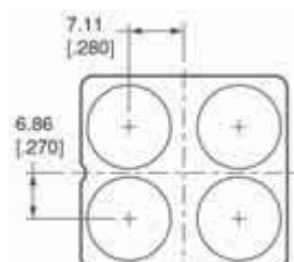
ARINC 600, 4 Position 4MP
