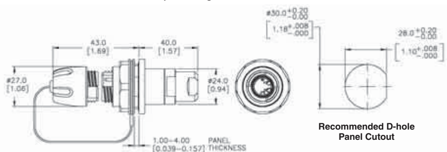
PRO BEAM Jr. D-Hole Bulkhead, Standard Cable Adapter
