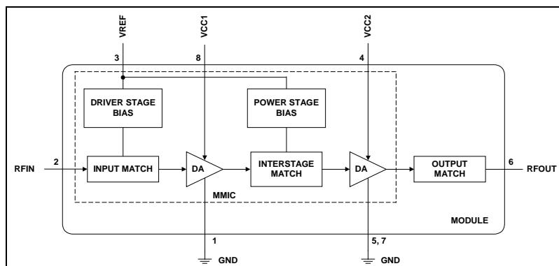
Figure 1. CX65105 Functional Block Diagram
