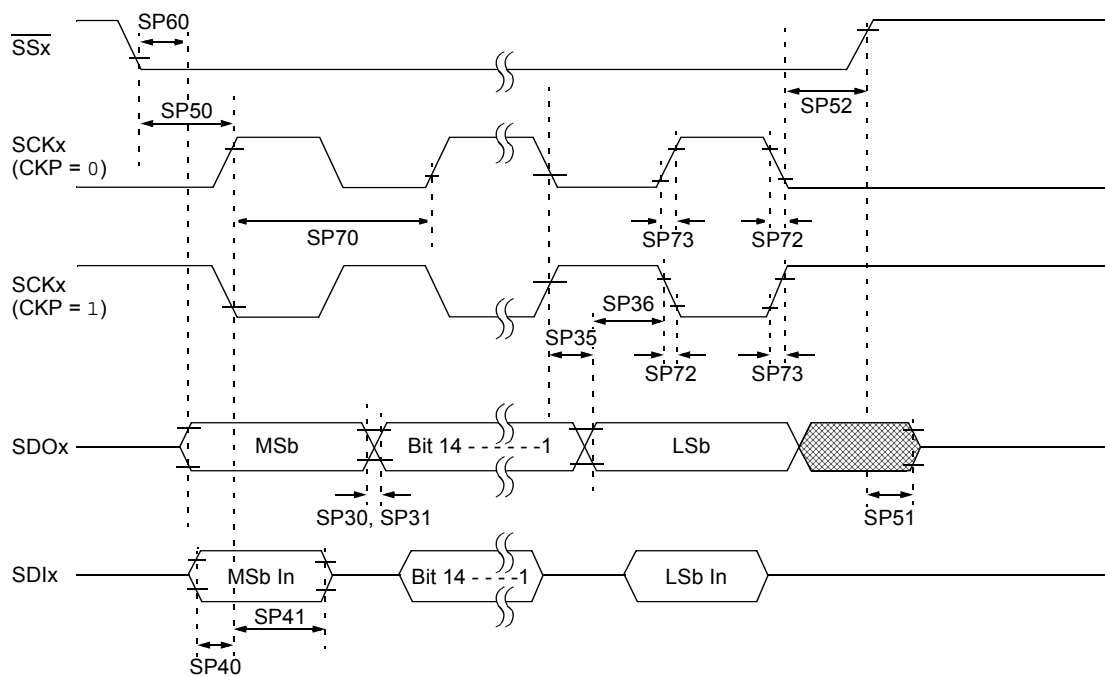
FIGURE 26-16: SPIx SLAVE MODE (FULL-DUPLEX, CKP = 1, CKP = 1, SMP = 0) TIMING CHARACTERISTICS
