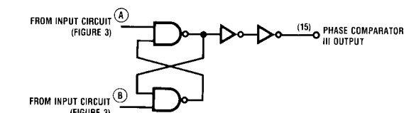
FIGURE 7. Phase Comparator III Logic Diagram
