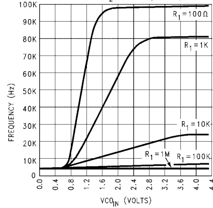
VHC4046 \text{VCO}_{\text{IN}} vs f_{\text{OUT}} \text{V}_{\text{CC}} = 4.5\text{V}
