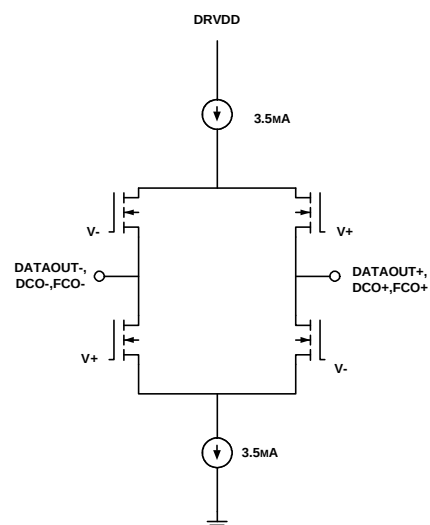
Figure 4 LVDS Outputs
