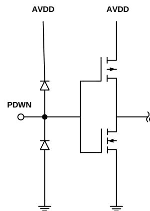
Figure 5 PDWN Input
