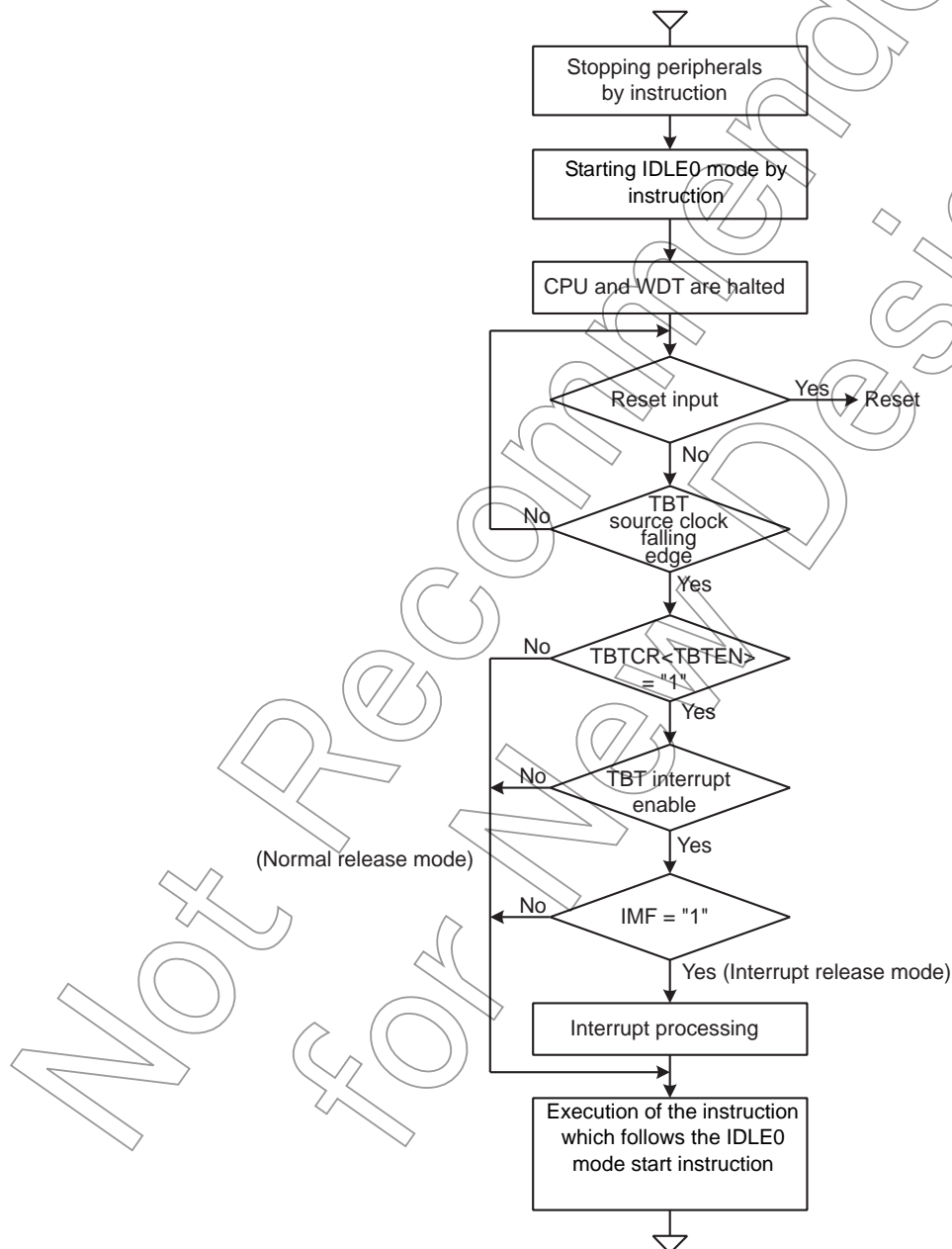
Figure 2-12 IDLE0 Mode
