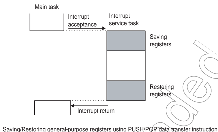
Figure 3-4 Saving/Restoring General-purpose Registers under Interrupt Processing
