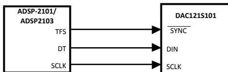
Figure 37. ADSP-2101/2103 Interface
