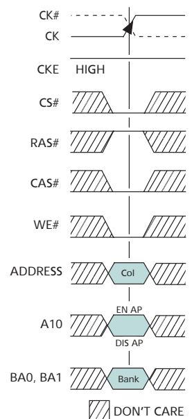
Figure 17: WRITE Command
