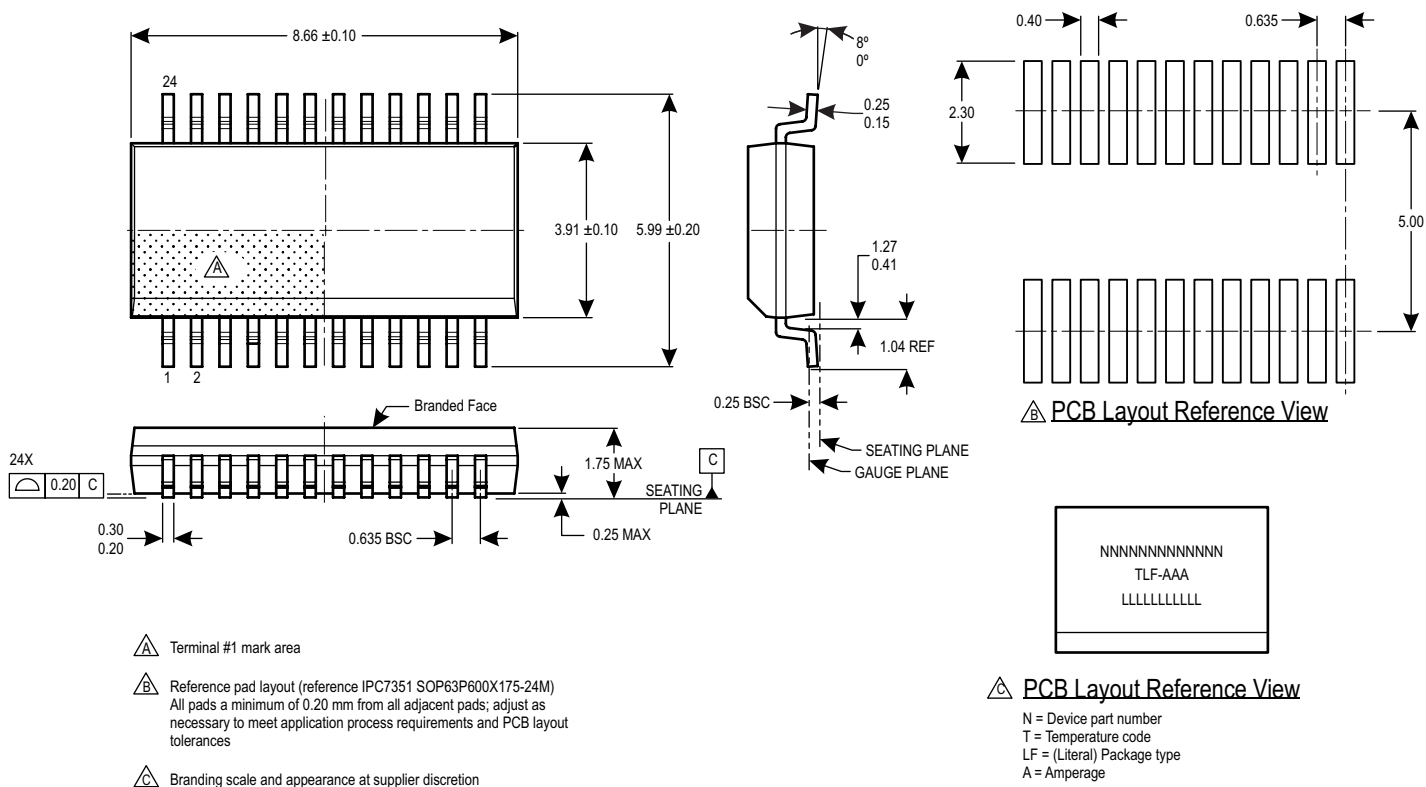
Package LF, 24-Pin QSOP
