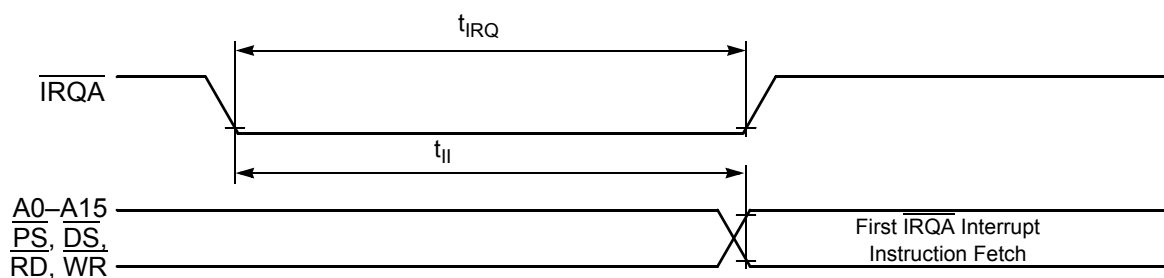
Figure 3-19 Recovery from Stop State Using \overline{IRQA} Interrupt Service
