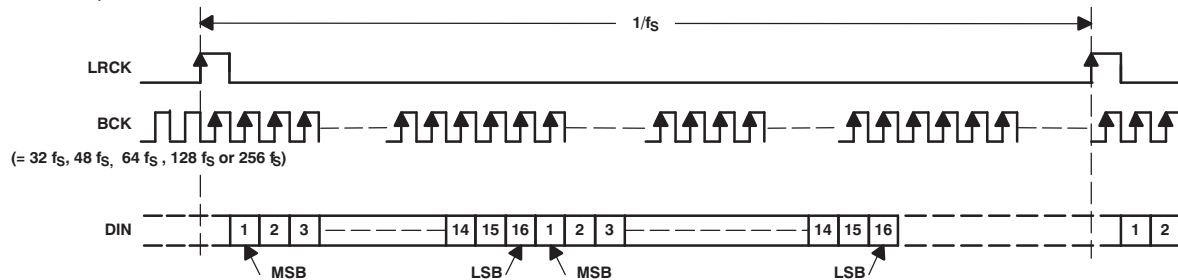
Figure 16. Audio Data Formats
