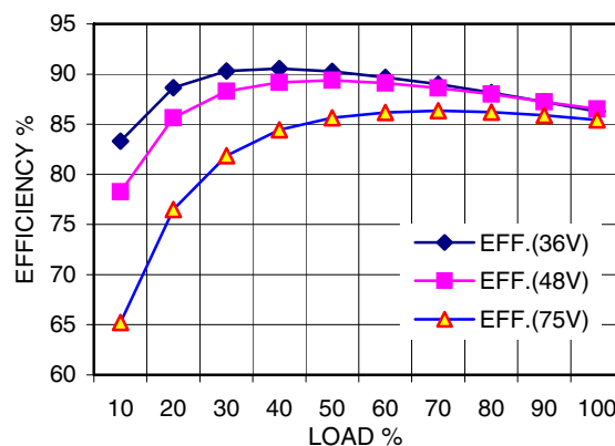
Figure 3. QHS40ZD Efficiency vs. Output Load
