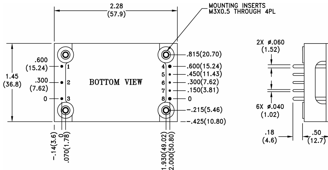
Figure 15. Mechanical Drawing
