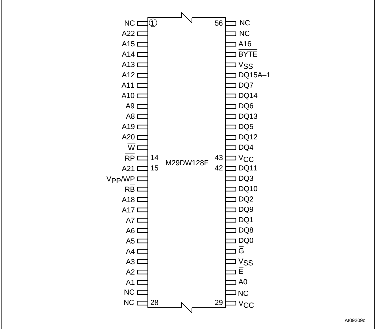
Figure 2. TSOP connections
