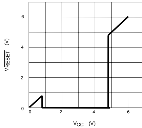
\overline{\text{RESET}} output characteristics
