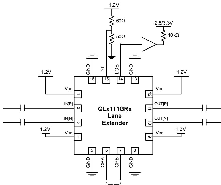
FIGURE 8. TYPICAL APPLICATION REFERENCE DESIGN
