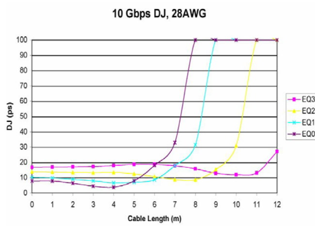
FIGURE 2. JITTER vs CABLE LENGTH AT 10Gb/s (BOOST LEVELS 0-3)
