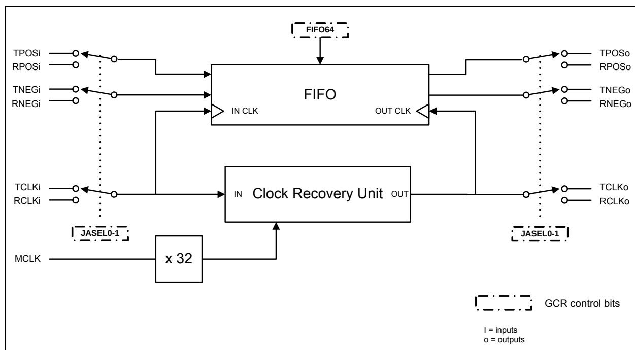
Figure 7 Jitter Attenuator
