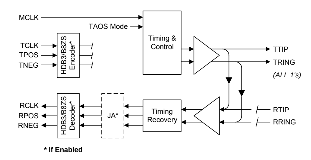
Figure 12 TAOS with Analog Loopback for LXT384 Transceiver
