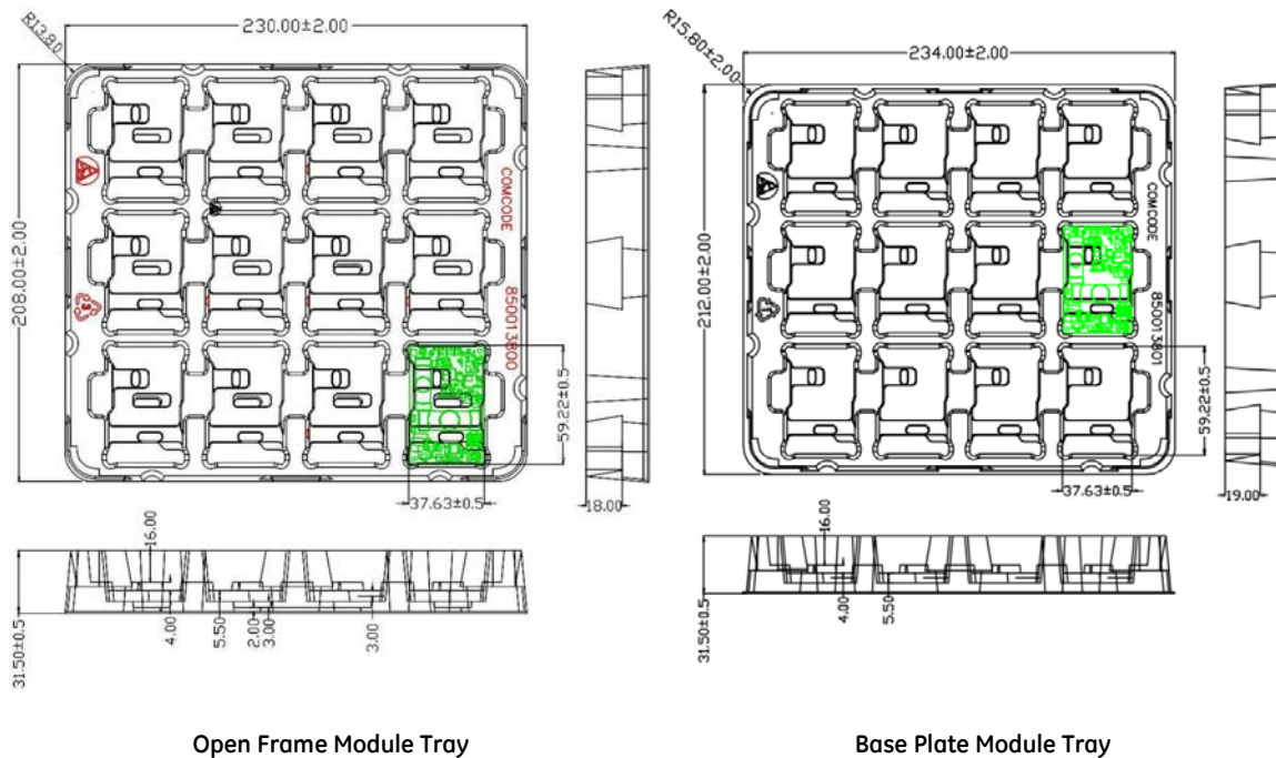
Figure 27. QBVW025 Packaging Tray
