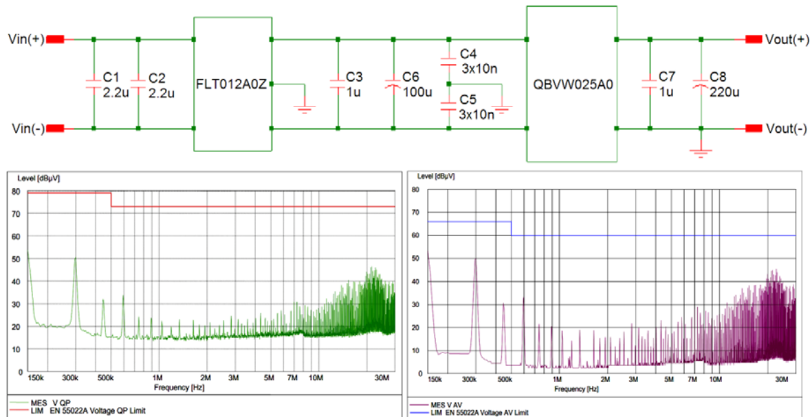
Figure 26. EMC Considerations
