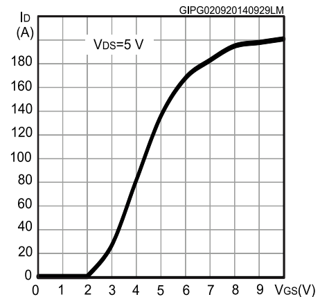
Figure 4. Transfer characteristics
