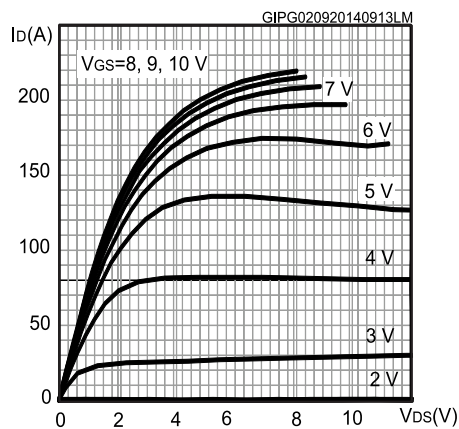
Figure 3. Output characteristics
