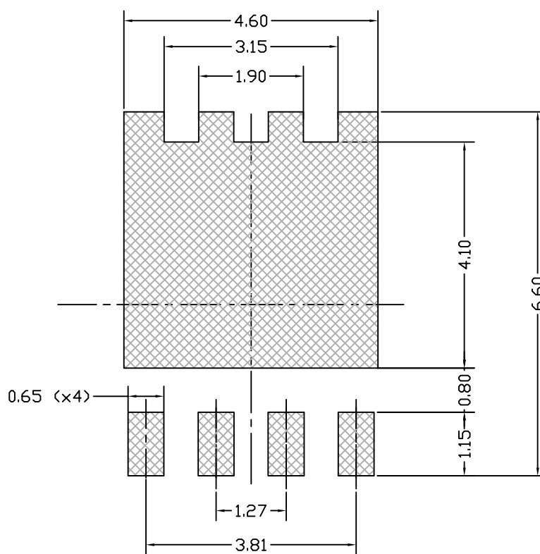
Figure 17. PowerFLAT 5x6 recommended footprint (dimensions are in mm)
