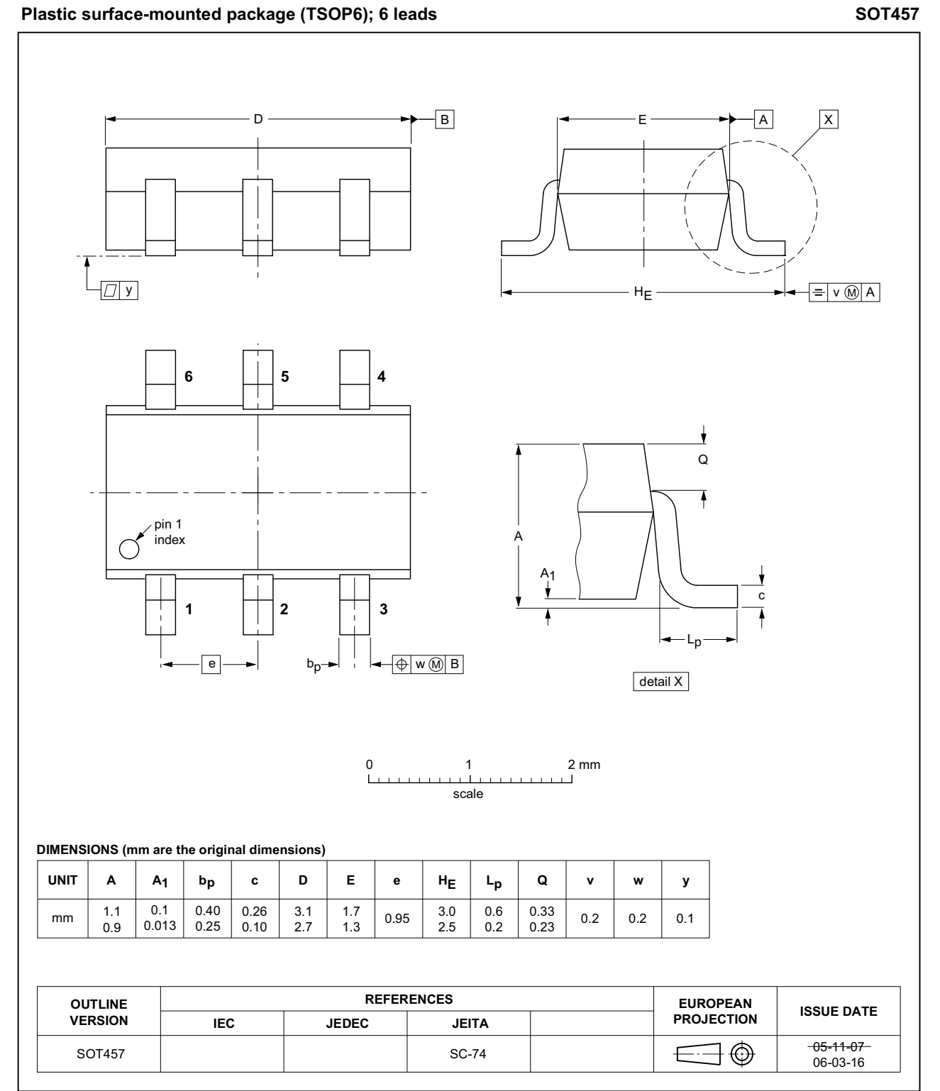
Fig 10. Package outline SOT457 (SC-74)
