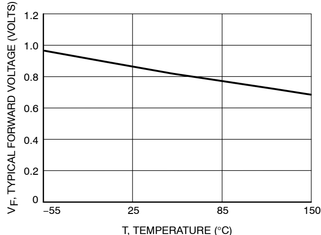
Figure 7. Forward Voltage
