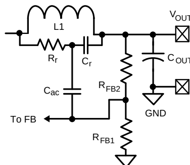
Figure 20. Type III Feedback Ripple Circuit
