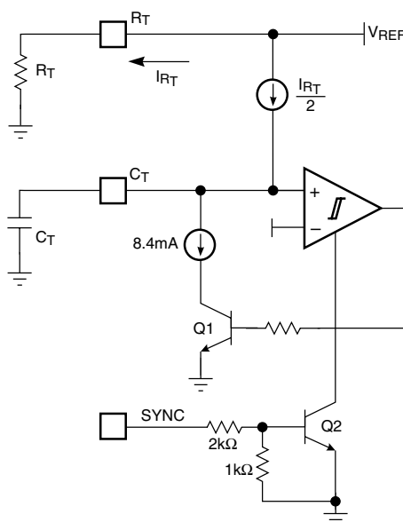
Figure 1. Oscillator Block Diagram
