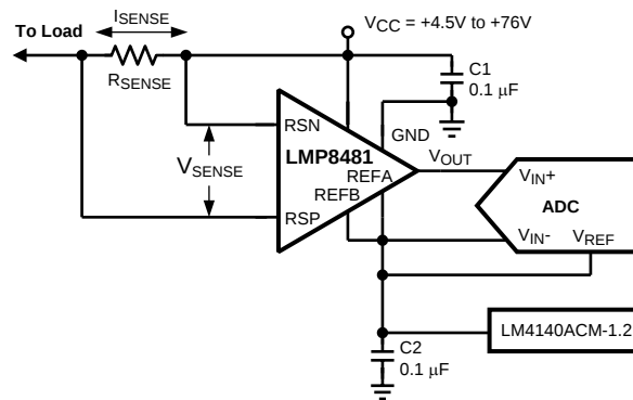
Figure 10. Bi-Directional current sensing using LMP8481
