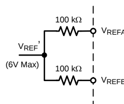
Figure 12. V_{REF} Input Resistor Network
