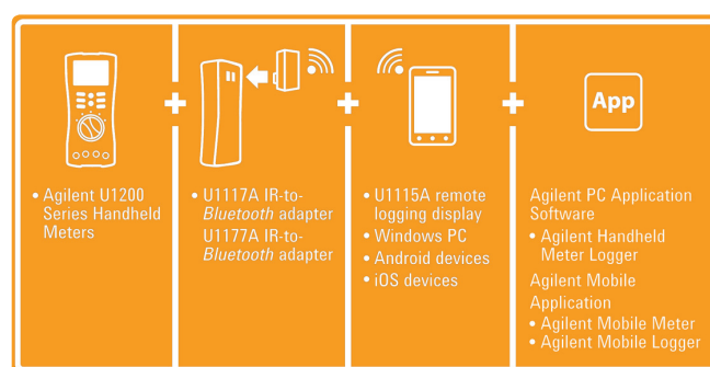
Figure 8. Agilent remote link solution
