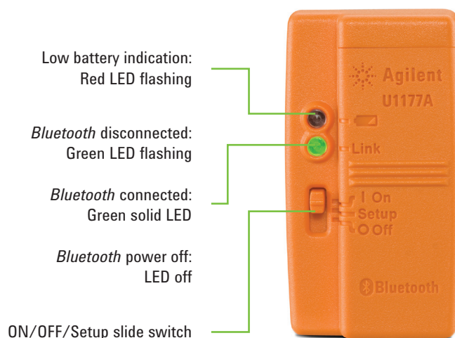
Figure 5. The U1177A as illustrated
